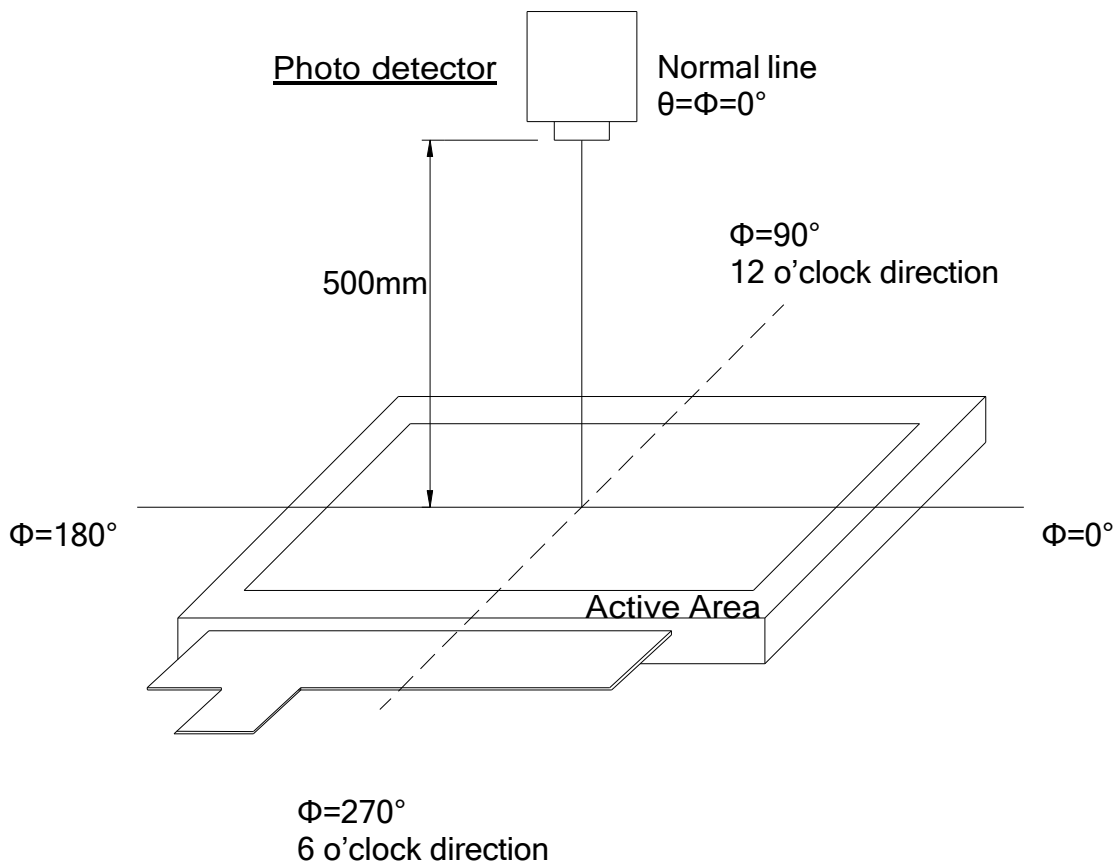
Fig. 4-2 Optical measurement system setup
