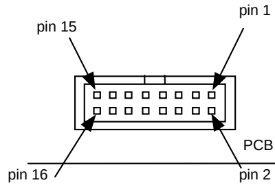
Parallel I/F connector IRISO: IMSA-9032B-16P or equivalent
