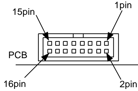
Parallel I/F & Power connector IRISO: IMSA-9032B-16P or Equivalent
