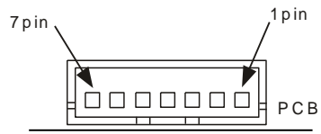
RS-232 I/F & Power connector JST: B7B-XH-A or equivalent
