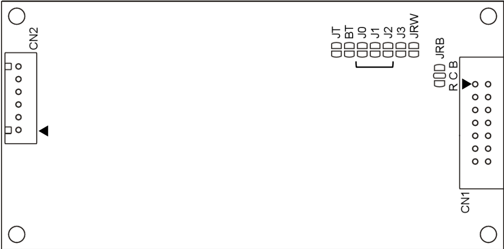
Parts side view. JT, BT, JRW: Factory use only.
